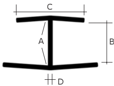
UNEQUAL H SECTION
